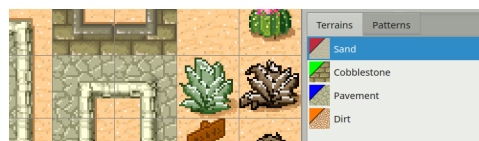
Abb. 3: Our Terrains
